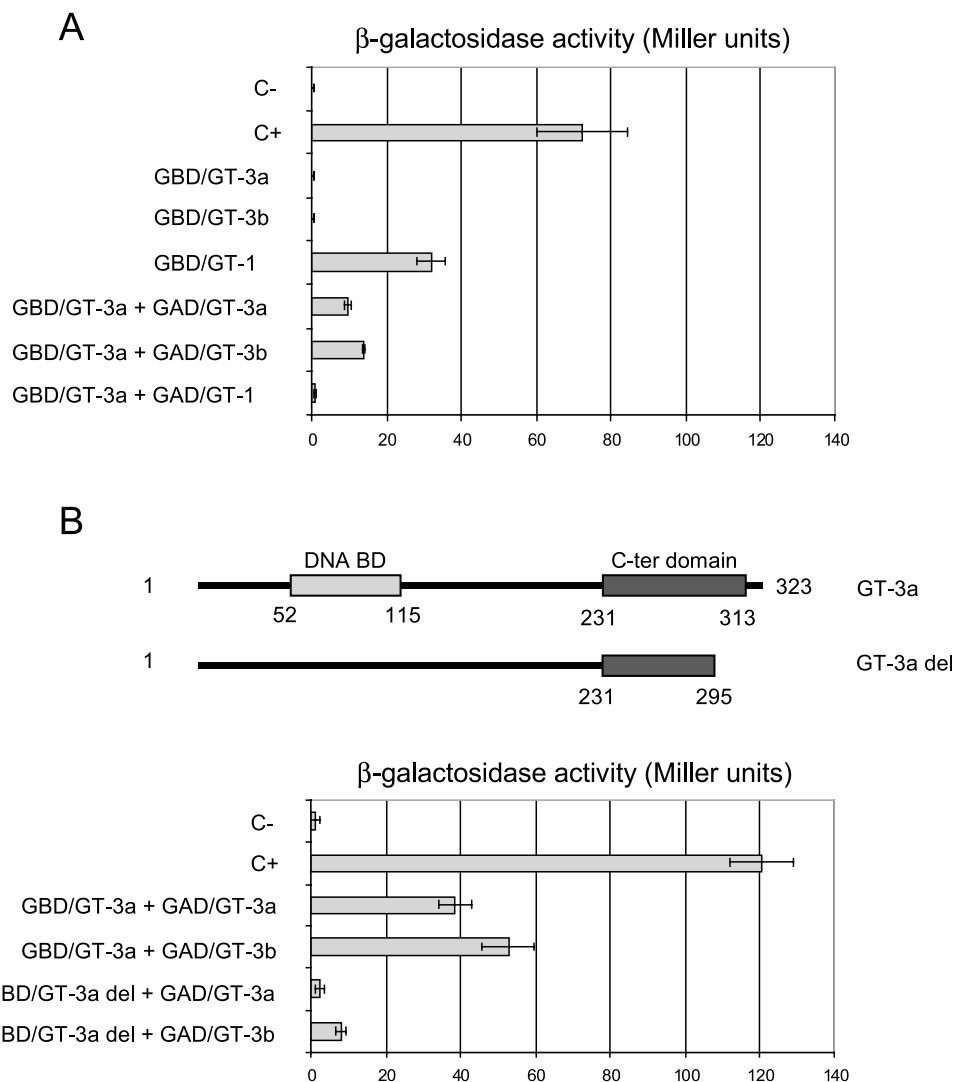
Fig. 2. Two-hybrid analysis of protein interaction between GT-3a and other GT factors in yeast. A: Average values of β-galactosidase activities measured from three independent transformations with combinations of bait (GBD/protein X) and prey (GAD/protein Y) constructs. B: Two-hybrid assays achieved with the GT-3a truncated protein (GT-3a del). C–: negative control (GAL 4 DNA-binding domain); C+: positive control (GAL 4 protein).
